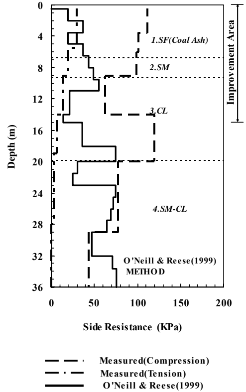
Fig. 12 Measured and estimated skin resistance along shafts
