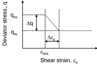
Fig. 3 An empirical shear strain versus deviator stress relationship
