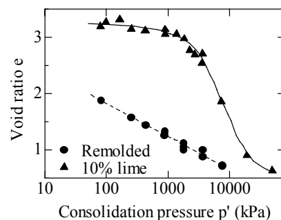
Fig. 16 e - \ln(p') curves of remoulded and lime stabilized samples
