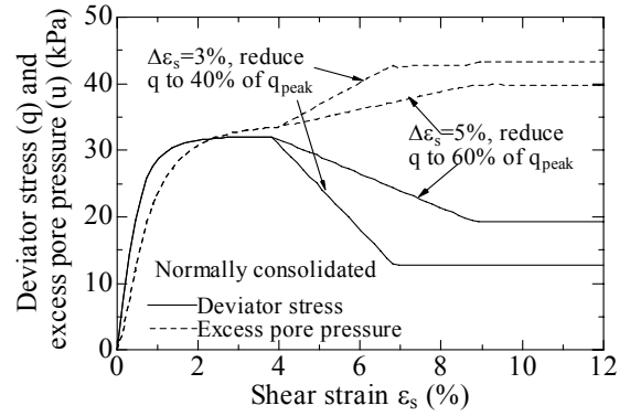
Fig. 5 \epsilon_s - q and \epsilon_s - u curves (NC)
