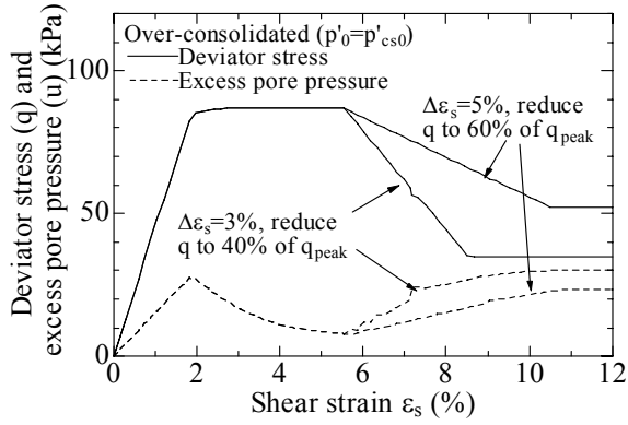
Fig. 9 \epsilon_s - q and \epsilon_s - u curves (OC-2)
