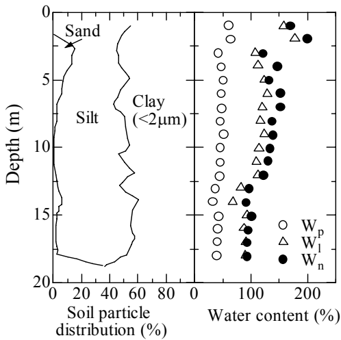
Fig. 11 Soil profile at Hizen-Kashima, Saga, Japan
