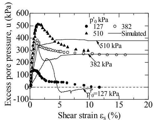
Fig. 19 Comparison of \epsilon_s - u curves of lime stabilized Ariake clay
