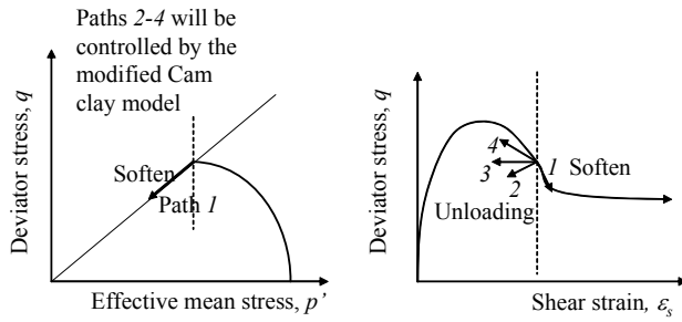
Fig. 2 Possible stress paths after stress state passes the peak
