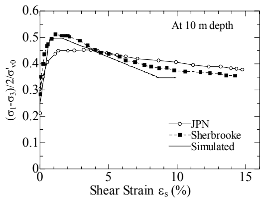
Fig. 13. Comparison of shear strain versus normalized deviator stress curves of undisturbed Ariake clay
