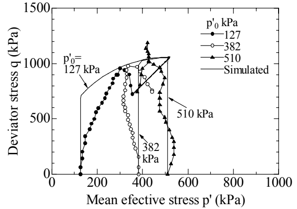
Fig. 18 Comparison of effective stress paths of lime stabilized Ariake clay
