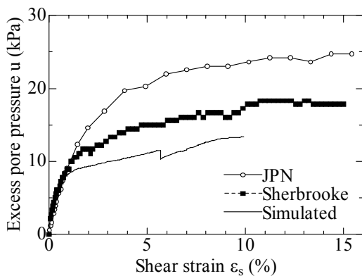
Fig. 15 Comparison of excess pore pressure variation
