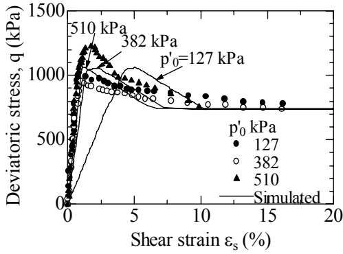
Fig. 17 Comparison of \epsilon_s - q curves of lime stabilized Ariake clay
