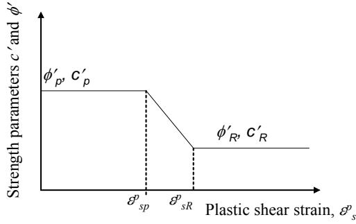
Fig. 1 Empirical strength/shear strain relationship
