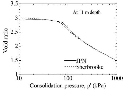
Fig. 12. Consolidation curves for the samples at 11 m depth (data points from Tanaka, 2000).
