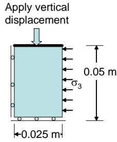
Fig. 4 Element size and boundary conditions
