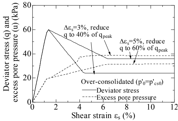
Fig. 7 \varepsilon_s - q and \varepsilon_s - u curves (OC-1)
