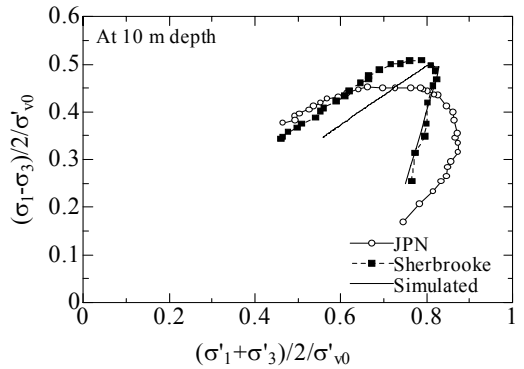
Fig. 14. Comparison of effective stress path of undisturbed Ariake clay
