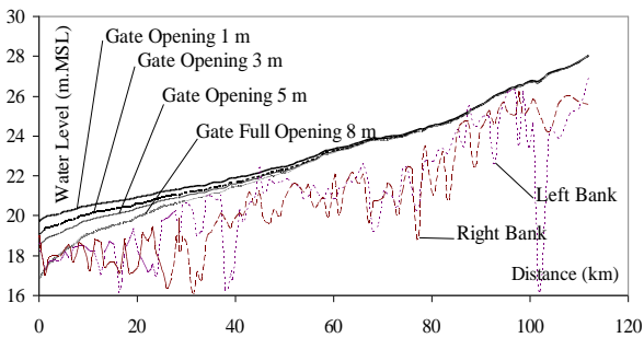
Fig.10 Highest water level along the Chao Phraya River in various cases of gate opening (use hydrological data in 1995 and assume no water diversion into the irrigation canals)
