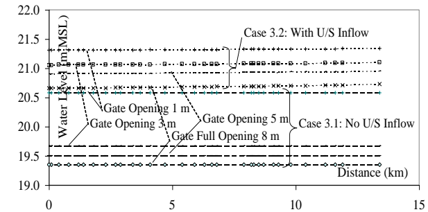
Fig.15 Comparison between the highest water level along the Sakaekang River in Case 3.1: No upstream inflow and Case 3.2: with upstream inflow
