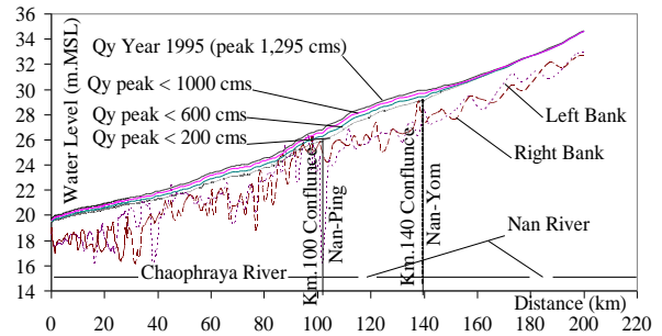
Fig.17 The highest water level along the Chao Phraya River in cases of controlling the peak discharge at Y.5: 200, 600, 1,000 cms and actual discharge in 1995
