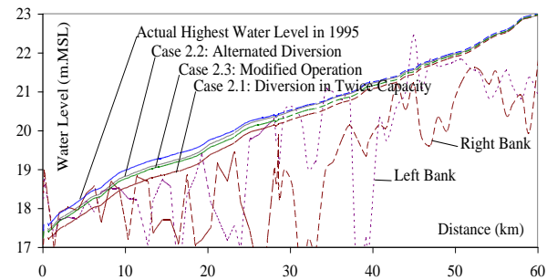
Fig.14 Comparison of the highest water level along the Chao Phraya River in Case 2.1, 2.2 and 2.3
