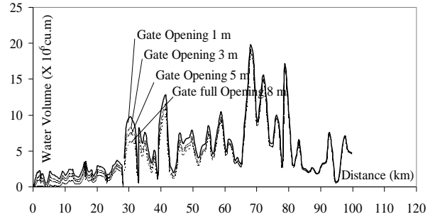
Fig.11 The volume of the flood inundation over riverbank along the Chao Phraya River at the highest water level in various cases of gate opening
