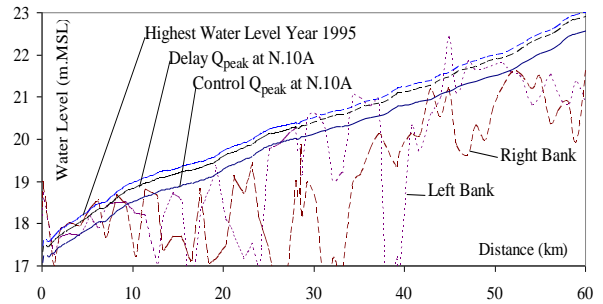
Fig.19 The highest water level along the Chao Phraya River in Case 5.1: the peak discharge (<1,500 cms) at N.10A and Case 5.2: delaying the peak discharge 14 days
