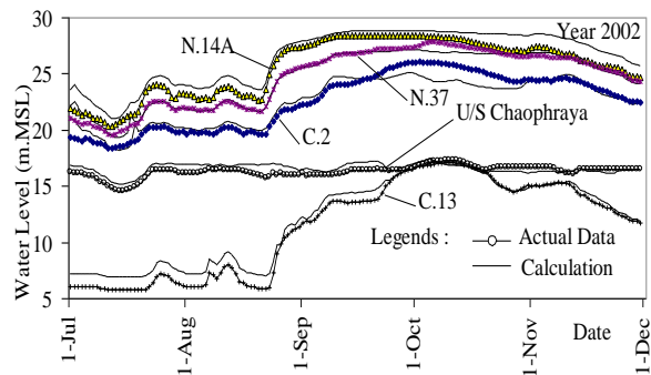
Fig.8 Comparison between actual and calculation water level in 2002 (for the model verification)
