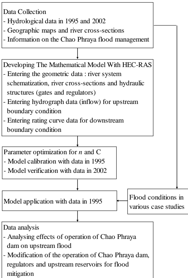
Fig.5 The schematic of the study approach
