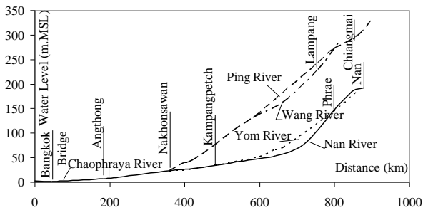
Fig.2 Profiles of the Chao Phraya River and the tributaries
