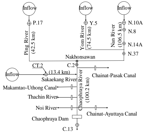
Fig.3 The schematic of the river network in the mathematical model
