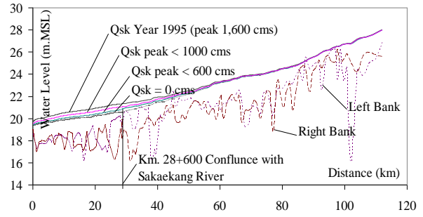
Fig.16 The highest water level along the Chao Phraya River in cases of controlling the peak discharge at CT.2: 0, 600, 1,000 cms and actual discharge in 1995
