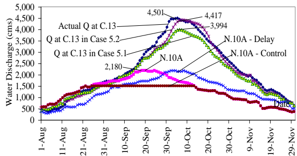
Fig.18 Comparison between water discharge at C.13 in Case 5.1: the peak discharge (<1,500 cms) and Case 5.2: delaying the peak discharge 14 days at N.10A
