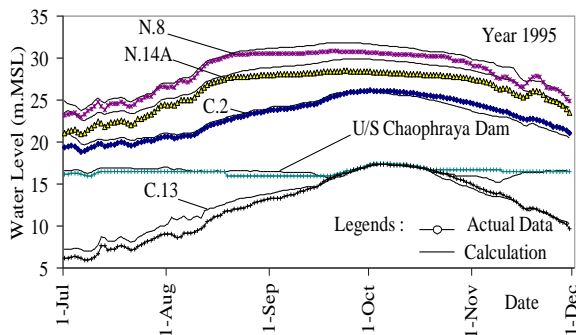
Fig.7 Comparison between actual and calculation water level in 1995 (for the model calibration)
