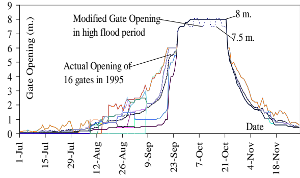
Fig.12 Comparison between the actual gate opening in 1995 and the modified gate opening in Case 2.3
