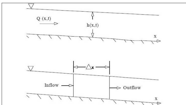
Fig.6 Elementary control volume for derivation of the continuity and momentum equations
