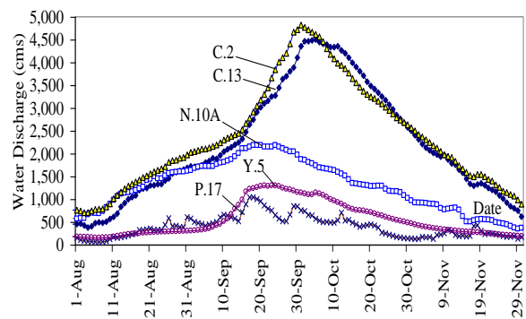
Fig.9 Flood hydrograph (data in 1995) from the river tributaries at P.17, Y.5, N.10A and the Chao Phraya River at C.2 and C.13
