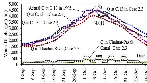
Fig.13 Comparison of water discharge at C.13 in Case 2.1, 2.2 and 2.3. And modified water diversion in the Thachin River and the Chainat-Pasak Canal in Case 2.3
