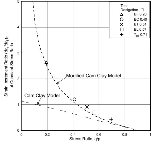
Fig. 4 Observed and predicted dilatancy ratio (Balasubramaniam, 1969)
