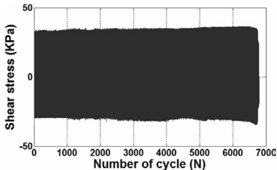
Fig. 5b. Shear Stress versus number of loading cycles with CSR = 0.2 at 15 % Double Amplitude Strain, ( \tau_a = 0\text{kPa} ) Symmetric loading \sigma'_{vc} = 200\text{ kPa} .
