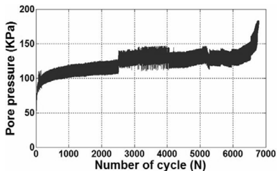
Fig. 5c. Excess Pore Pressure versus number of loading cycles with CSR = 0.2 at 15 % double amplitude strain, ( \tau_a = 0\text{ kPa} ) symmetric loading \sigma'_{vc} = 200\text{ kPa} .
