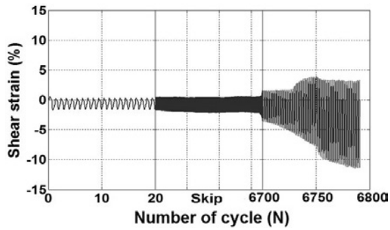
Fig. 5a. Shear Strain versus number of loading cycles with CSR = 0.3 at 15 % double amplitude strain, ( \tau_a = 0\text{kPa} ) symmetric loading \sigma'_{vc} = 200\text{ kPa}
