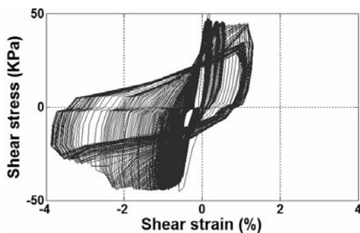
Fig. 6. Shear strain versus shear stress with CSR = 0.20 at 15 % double amplitude strain, ( \tau_a = 0\text{ kPa} ) symmetric loading, \sigma'_{vc} = 200\text{ kPa} .
